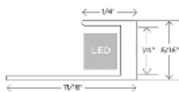
J SHAPED CHANNEL FRAME 5/16"
